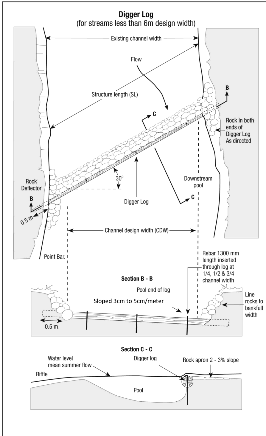
Conceptual drawing of a digger log (Thaumas Environmental Consultants Ltd.).
